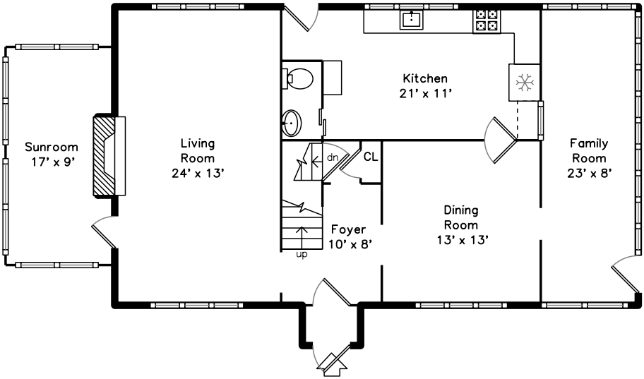
Main
