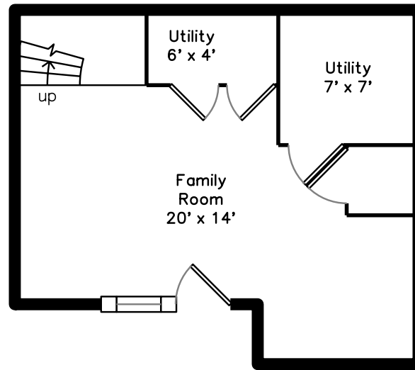
Basement
