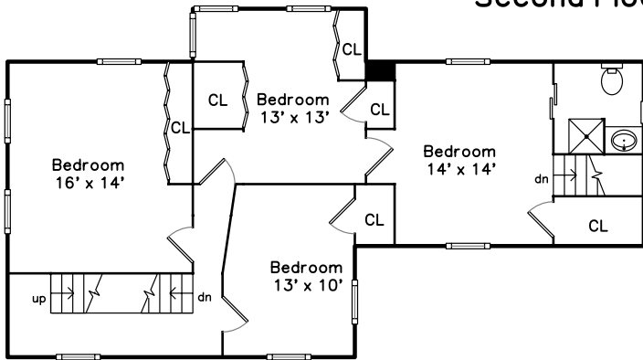
Second Floor
