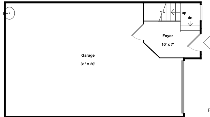
Garage/Entry
